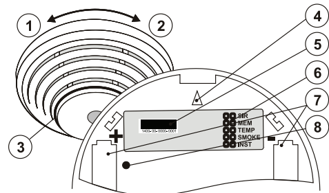
Fig 6: 1 – detector cover opening; 2 – detector cover closing; 3 – optical status signalling; 4 – arrow showing where to insert the detector; 5 – production code; 6 – configuration terminals; 7 – battery holders; 8 – button for test
